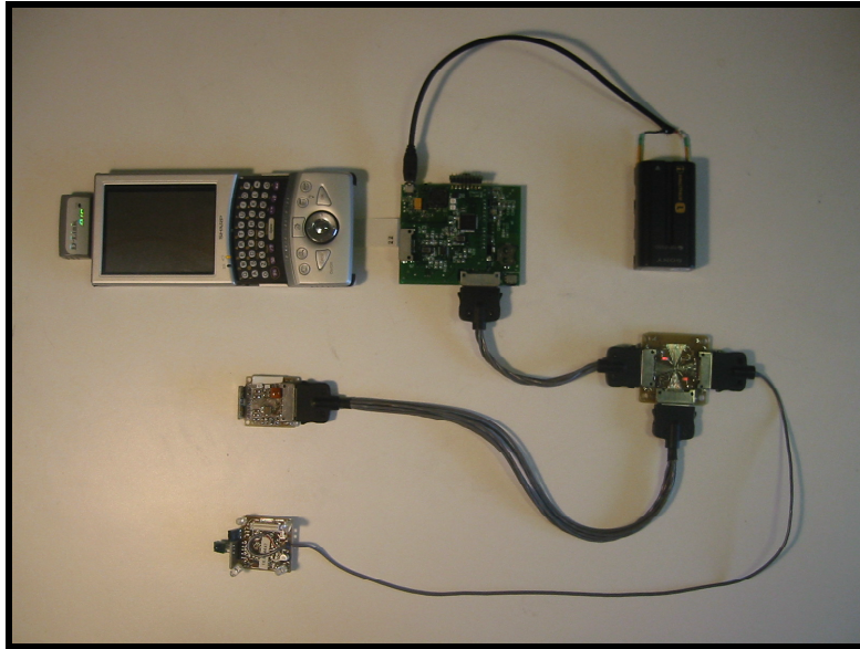
Figure 2: MIThril system, composed of the Zaurus PDA (top left), with SAK2 data acquisition/sensor hub and BioSense physiological sensing board with EKG/heart rate, skin conductance, temperature, respiration (middle), battery source (top right), sensor bus hub (lower right), motion-sensing board (middle left), and multisensor board with IR tag reader, audio, motion (lower left)
