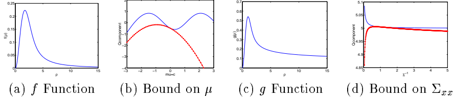
Figure 2: Bound Width Computation and Example Bounds
