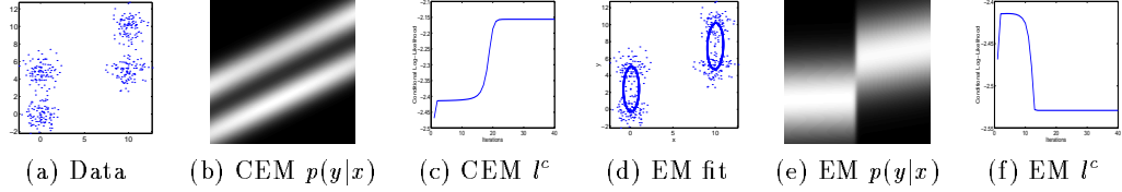
Figure 3: Conditional Density Estimation for CEM and EM
