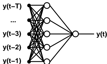
Figure 4.1: Static Network Representation of Temporal Modeling
