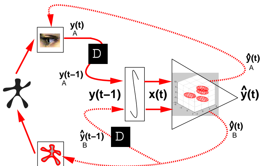
Figure 8.4: Perceptual Mode
