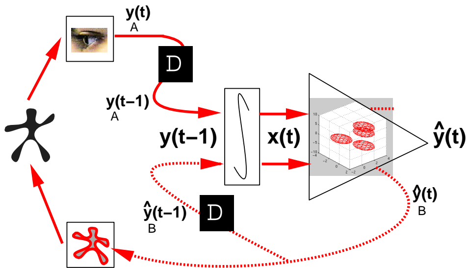
Figure 8.3: Interaction Mode
